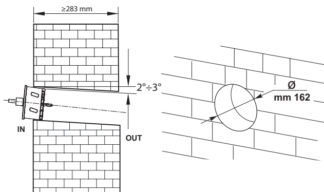
VORT HRW 40/60 MONO EVO -GRILLE MOUNTING FROM INSIDE
